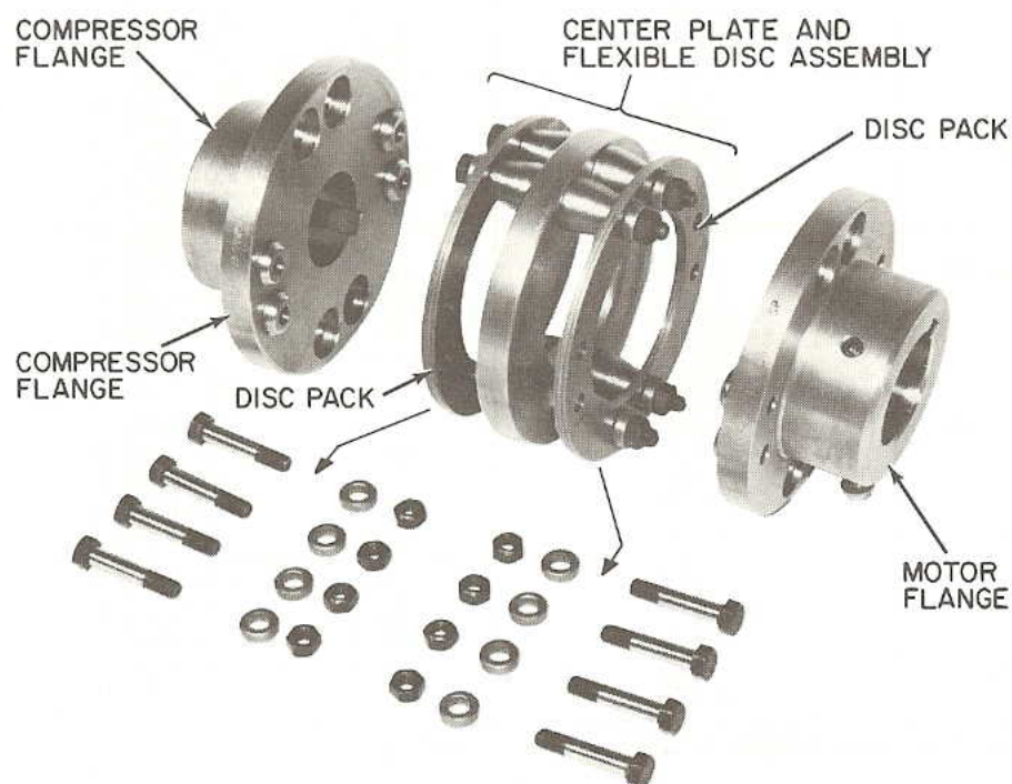
Fig. 3 — Disassembled Coupling
