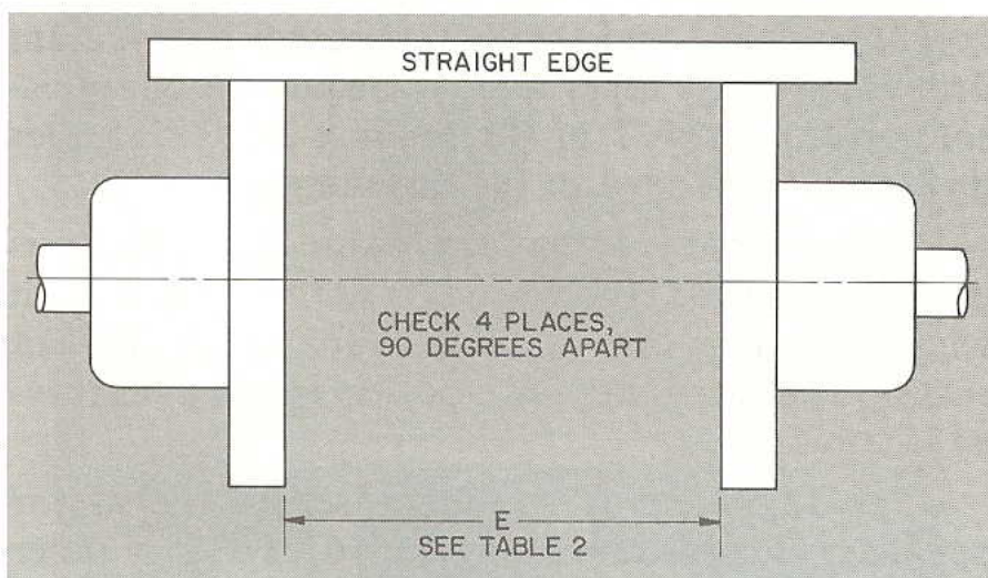
Fig. 4 — Preliminary Adjustment
