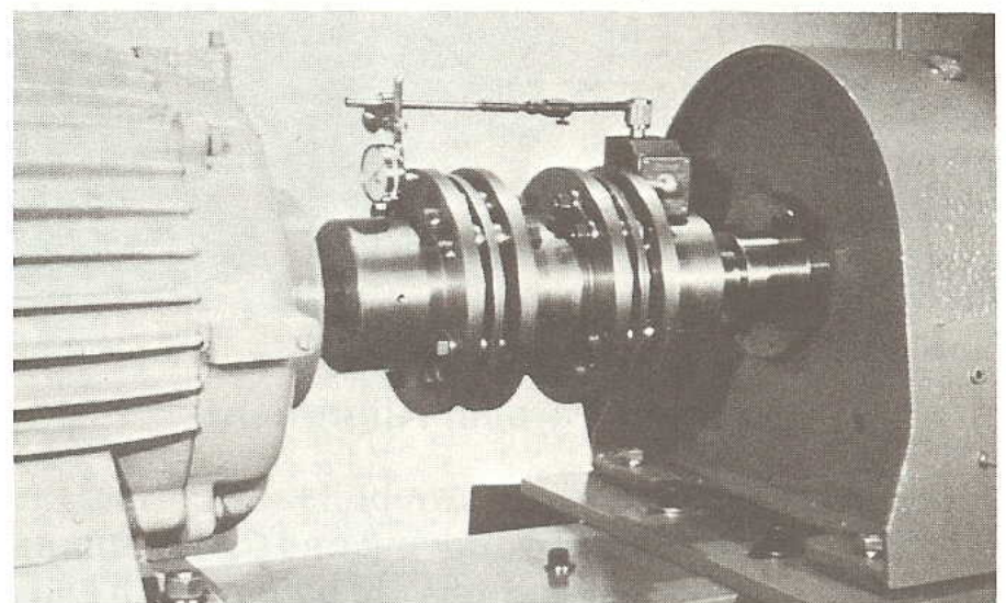
Fig. 5 — Set-Up for Checking Angular Alignment
