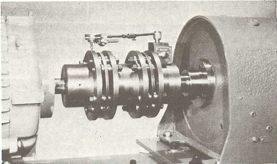
Fig. 6 — Set-Up for Checking Parallel Alignment
