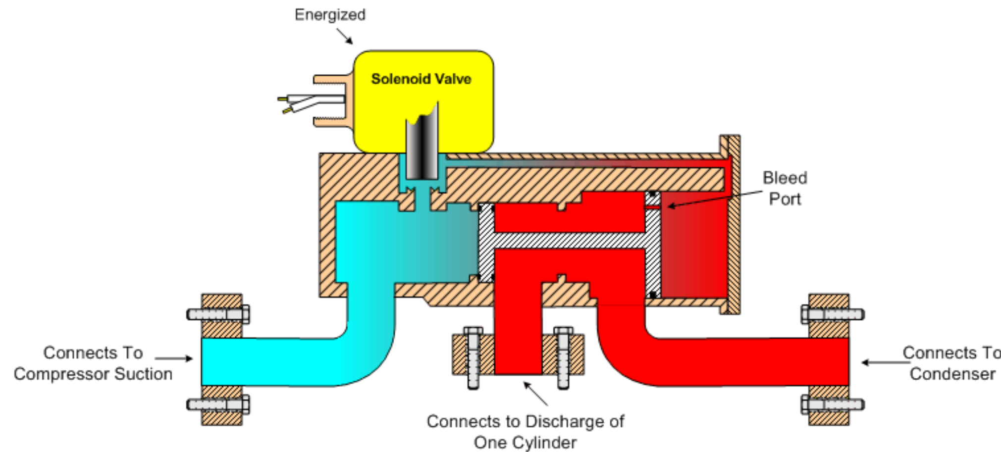
Unloader Valve in Loaded Position
