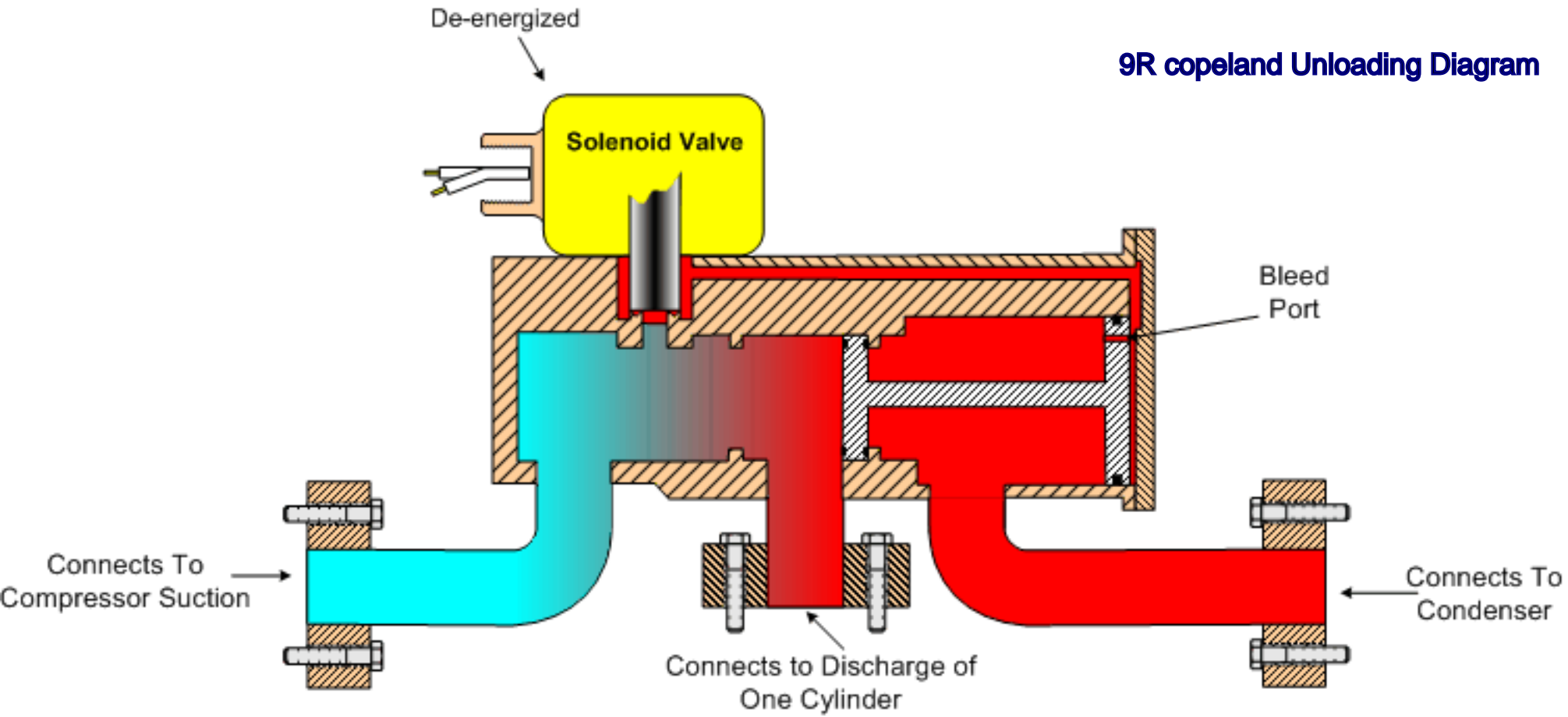
Unloader Valve in Unloaded Position
