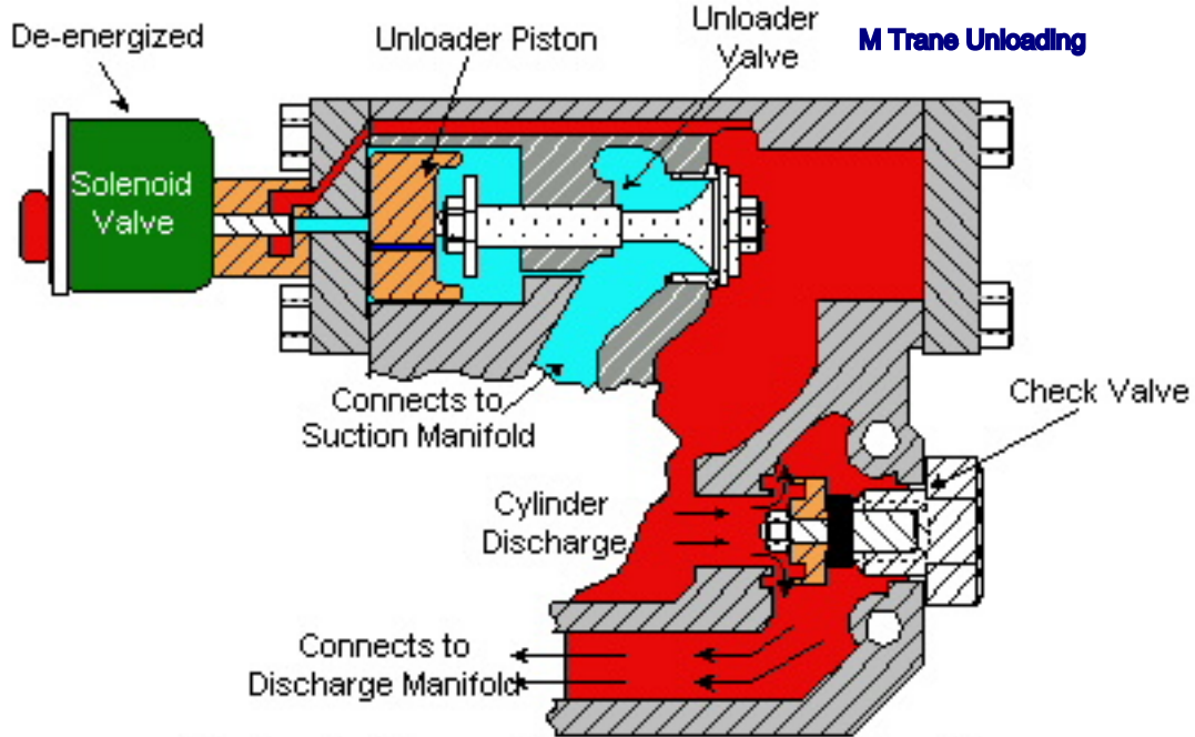
Unloader Piston & Valve in Loaded Position
