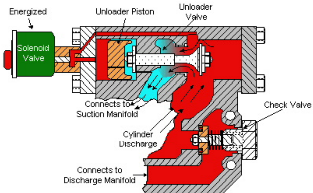
Unloader Piston & Valve in Unloaded Position
