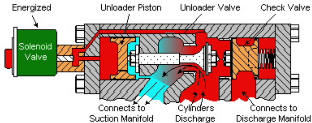
Unloader Piston & Valve in Unloaded Position
