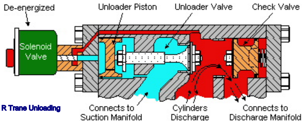
Unloader Piston & Valve in Loaded Position
